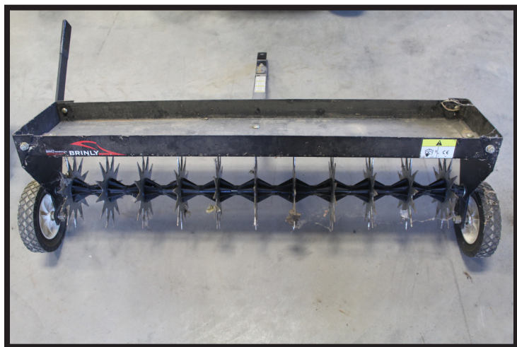
Pull-behind Aerator
